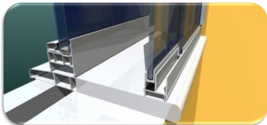
Cross cut drawing between existing Window (left) and installed secondary (right).
