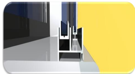
Cross cut drawing showing Horizontal Sliding secondary glazing.
